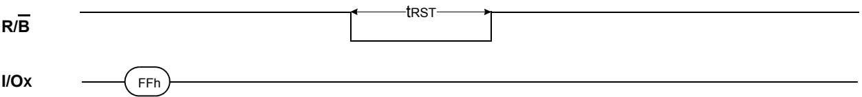
Figure 14. RESET Operation
