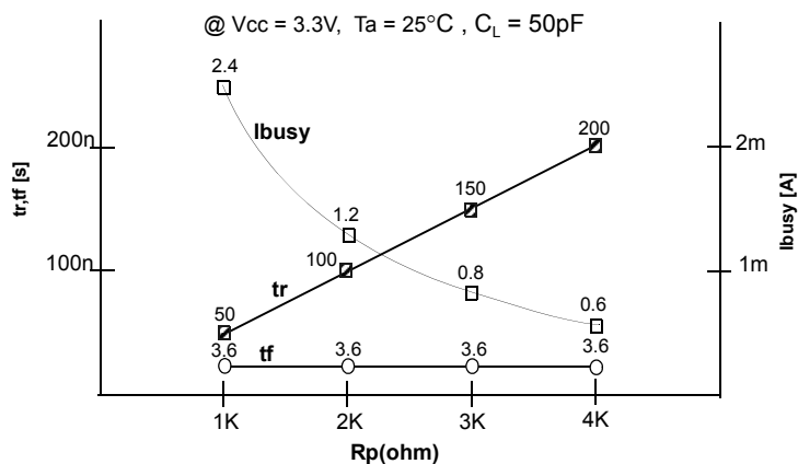
Figure 15. R_p vs t_r , t_f & R_p vs i_{\text{busy}}
